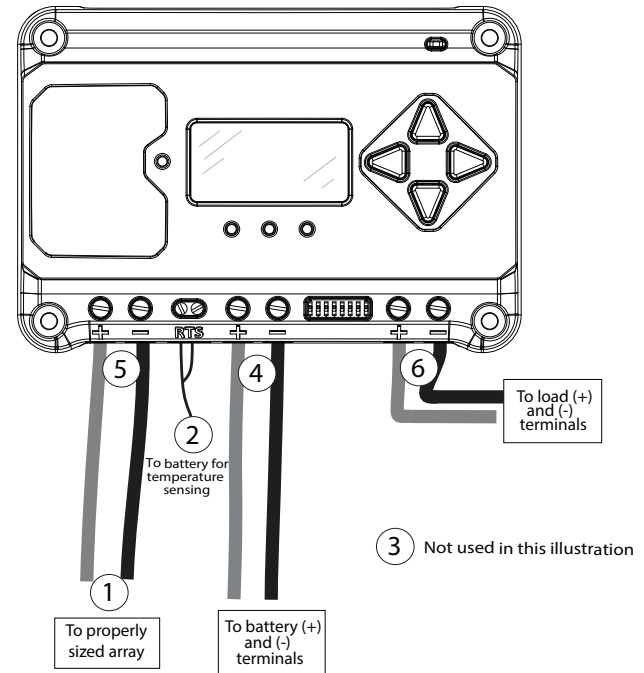
Figure 3-2. Wiring the EcoPulse
