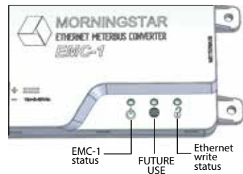
Figure 3-1. LED Indicators
