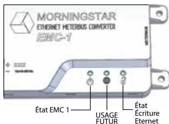
Figure 3-1. Voyants DEL
